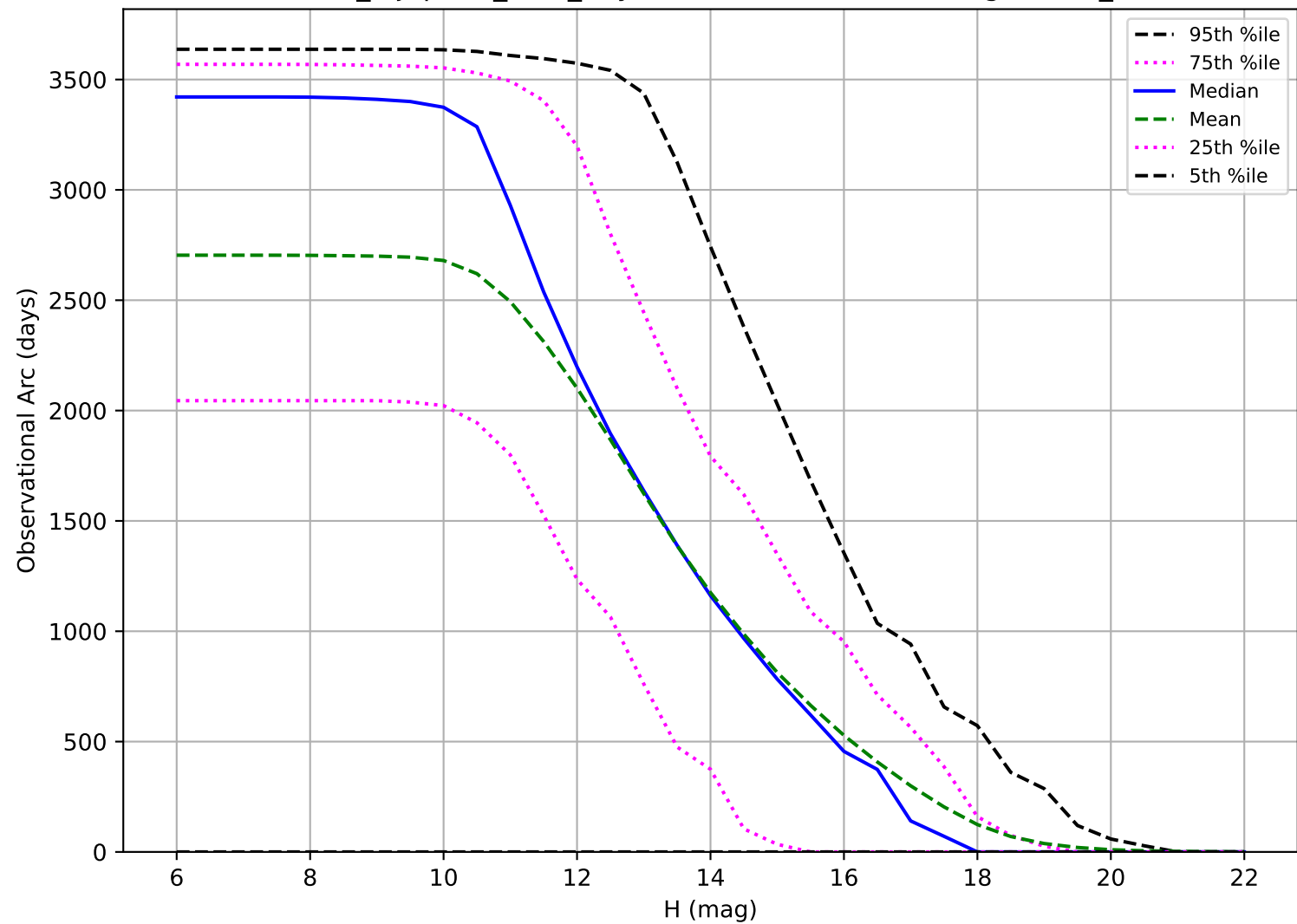
noroll_mjdp270_v3.4_10yrs: Observational Arc Length OCC_r5
