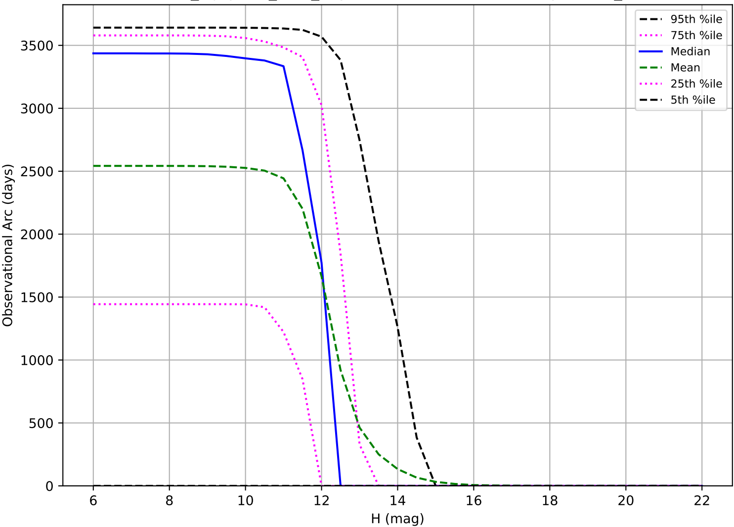
noroll_mjdp270_v3.4_10yrs: Observational Arc Length OCC_r20
