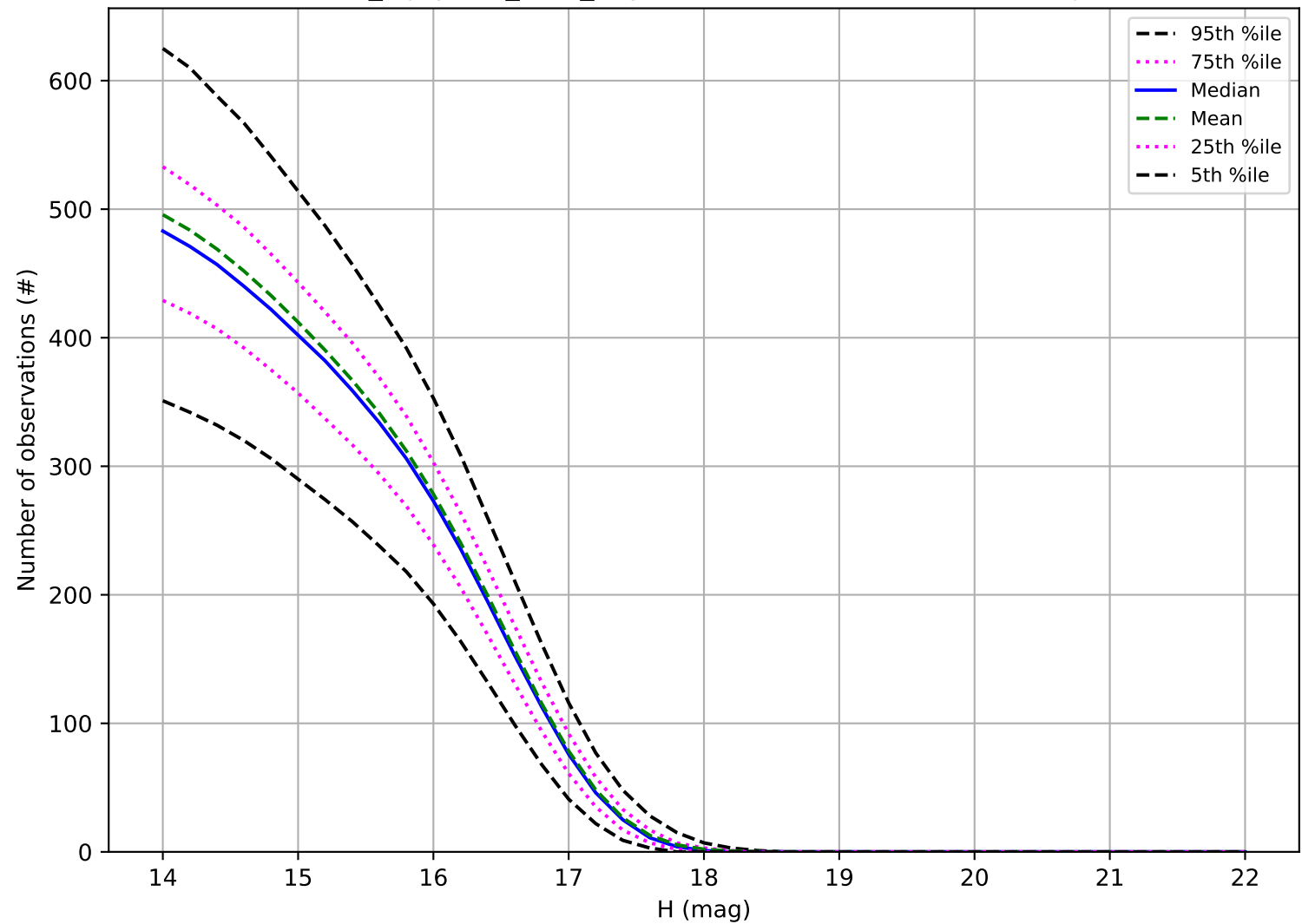
noroll_mjdp270_v3.4_10yrs: Number of observations Trojan
