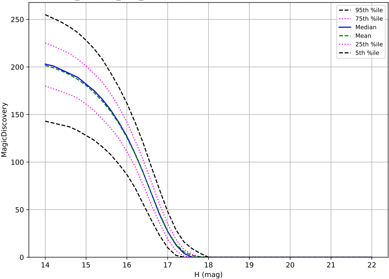
noroll_mjdp270_v3.4_10yrs: Trojan 6 detections in 60 nights detection loss
