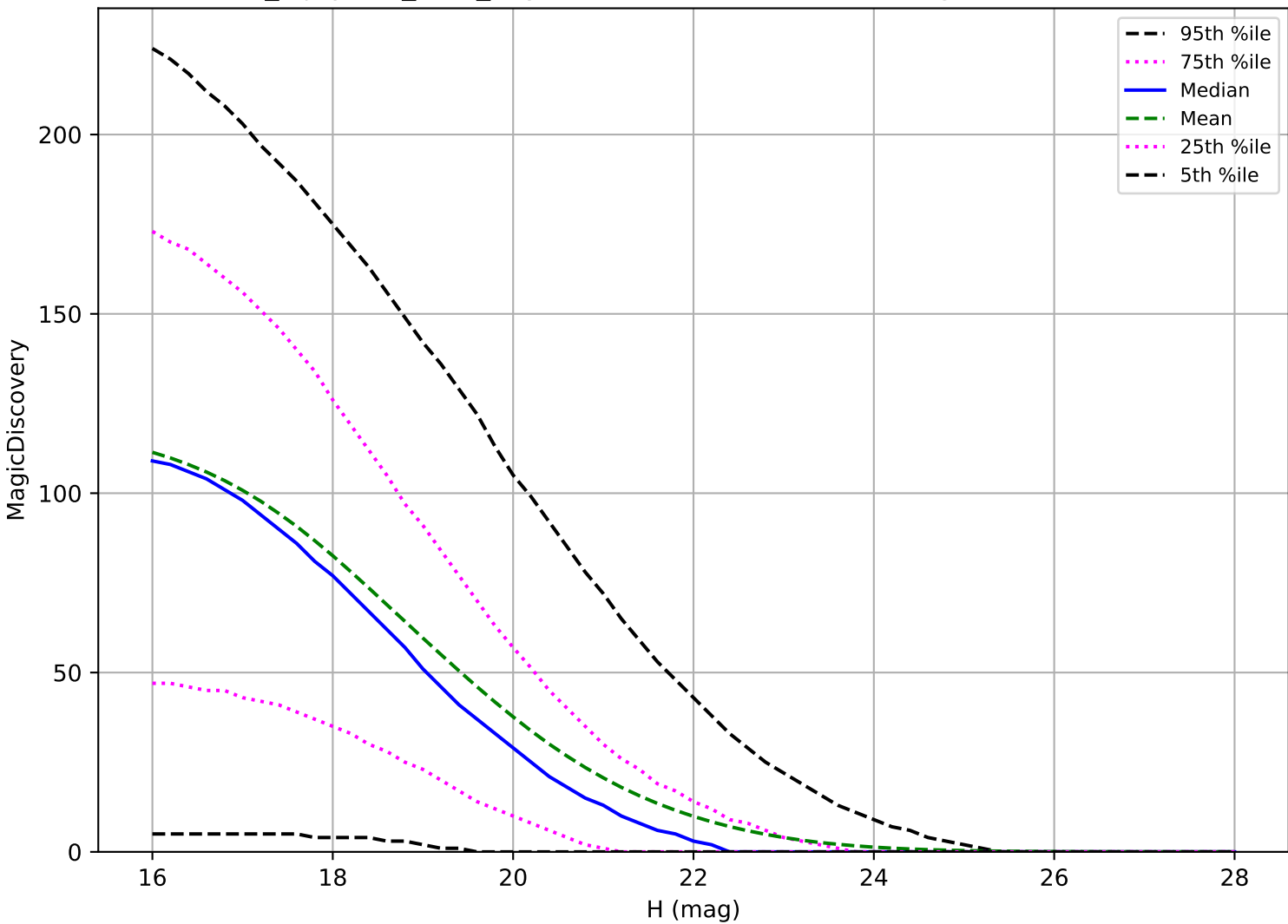
noroll_mjdp270_v3.4_10yrs: PHA 6 detections in 60 nights detection loss
