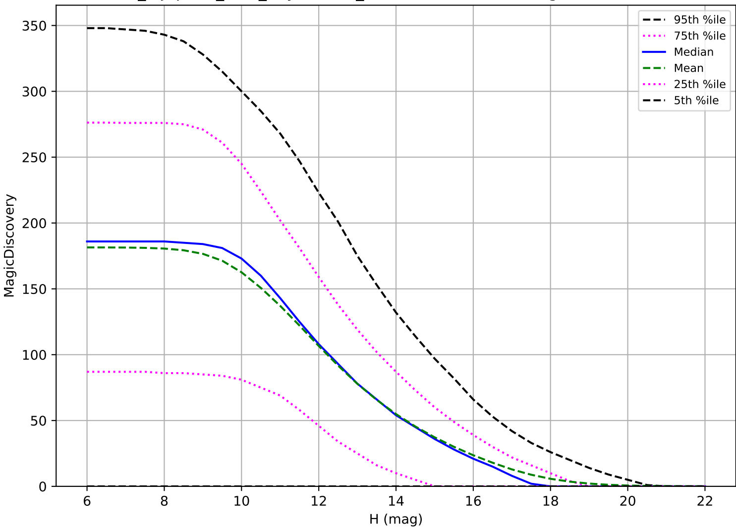
noroll_mjdp270_v3.4_10yrs: OCC_r5 6 detections in 60 nights detection loss
