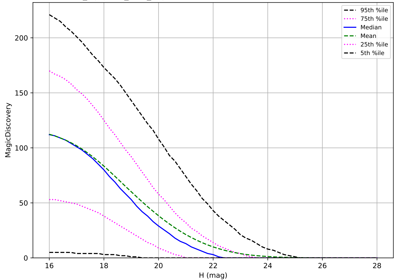
noroll_mjdp270_v3.4_10yrs: NEO 6 detections in 60 nights detection loss
