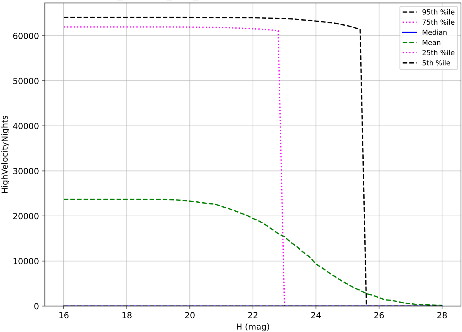
noroll_mjdp270_v3.4_10yrs: PHA High velocity pair detection loss
