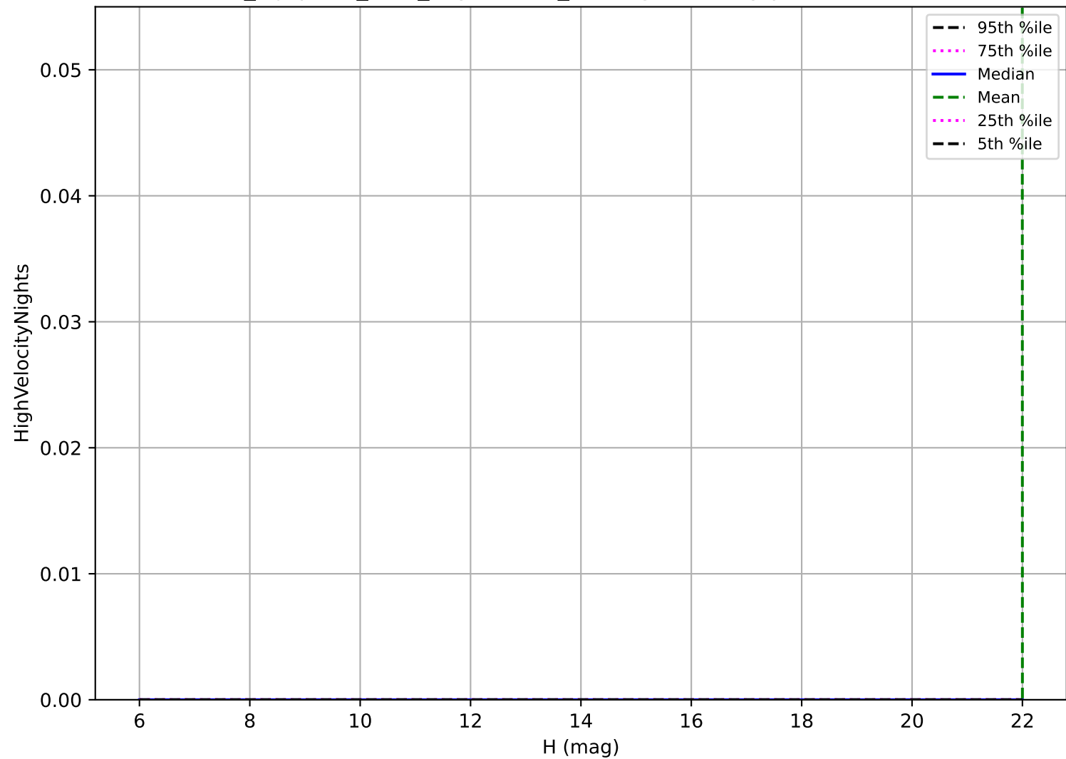
noroll_mjdp270_v3.4_10yrs: OCC_r20 High velocity pair detection loss
