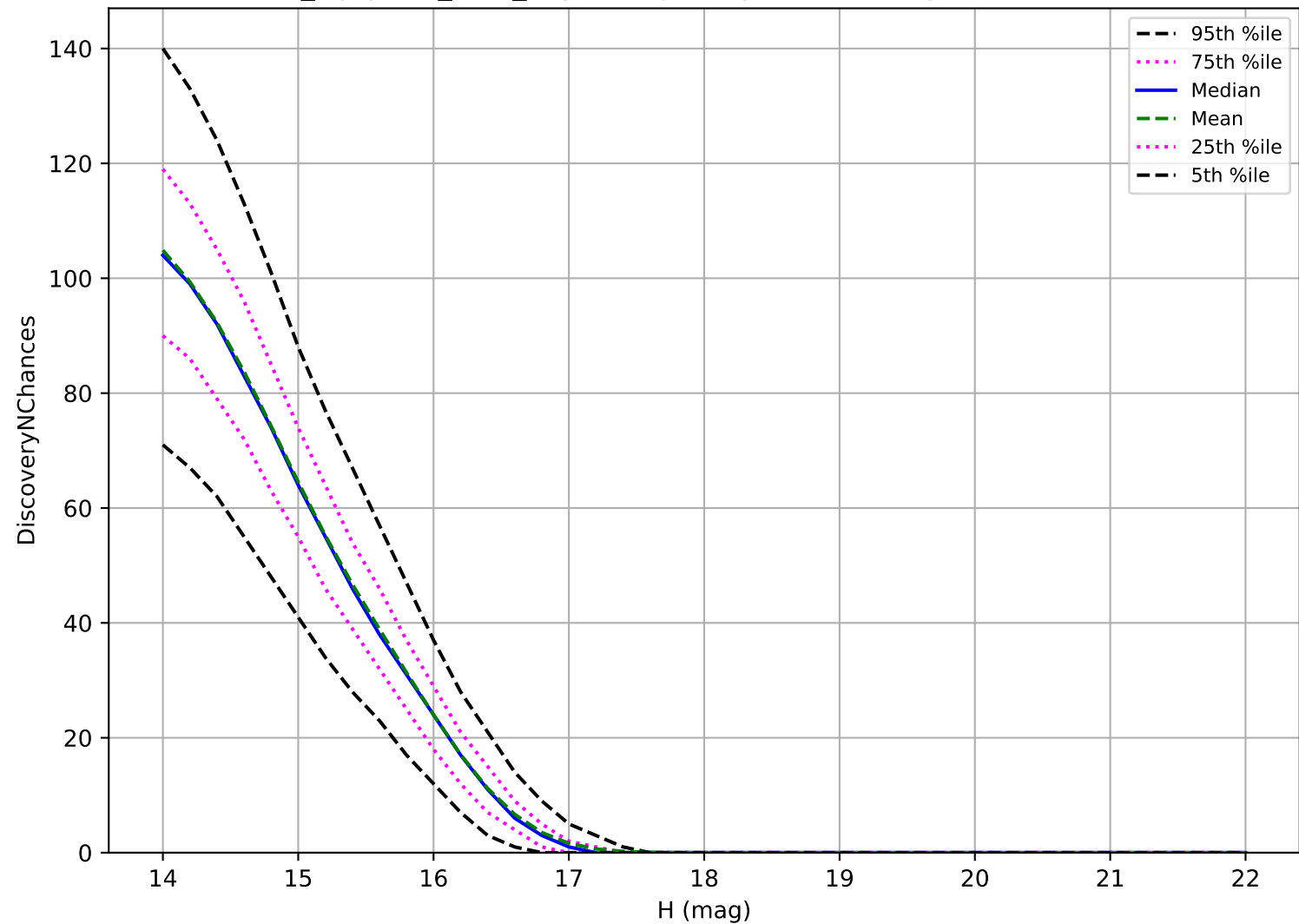
noroll_mjdp270_v3.4_10yrs: Trojan 3 pairs in 15 nights detection loss
