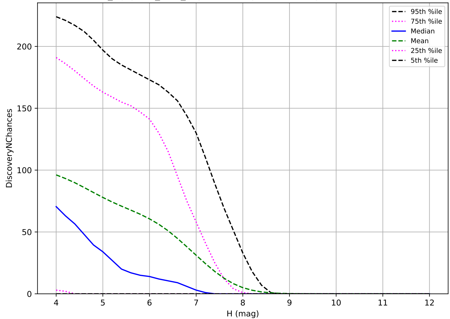
noroll_mjdp270_v3.4_10yrs: TNO 3 pairs in 15 nights detection loss
