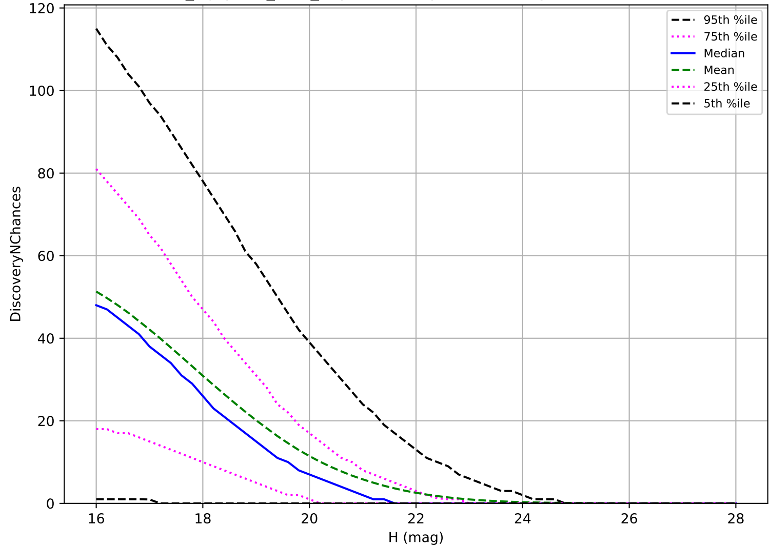
noroll_mjdp270_v3.4_10yrs: PHA 3 pairs in 15 nights detection loss
