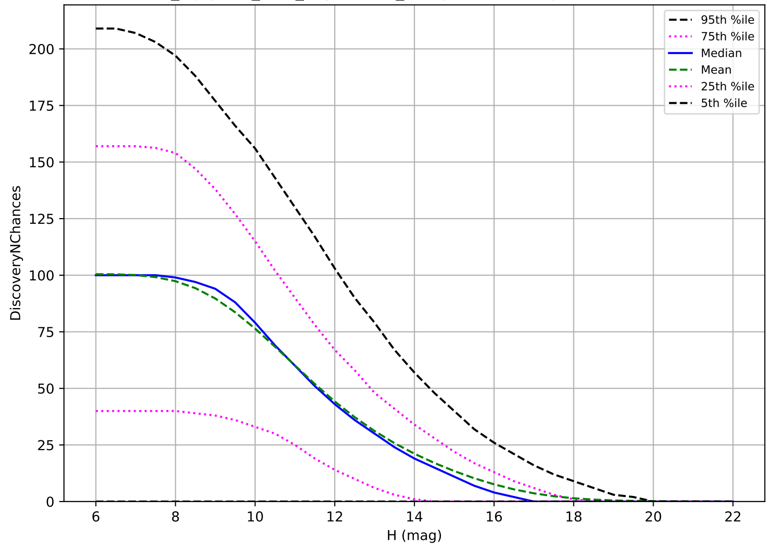
noroll_mjdp270_v3.4_10yrs: OCC_r5 3 pairs in 15 nights detection loss
