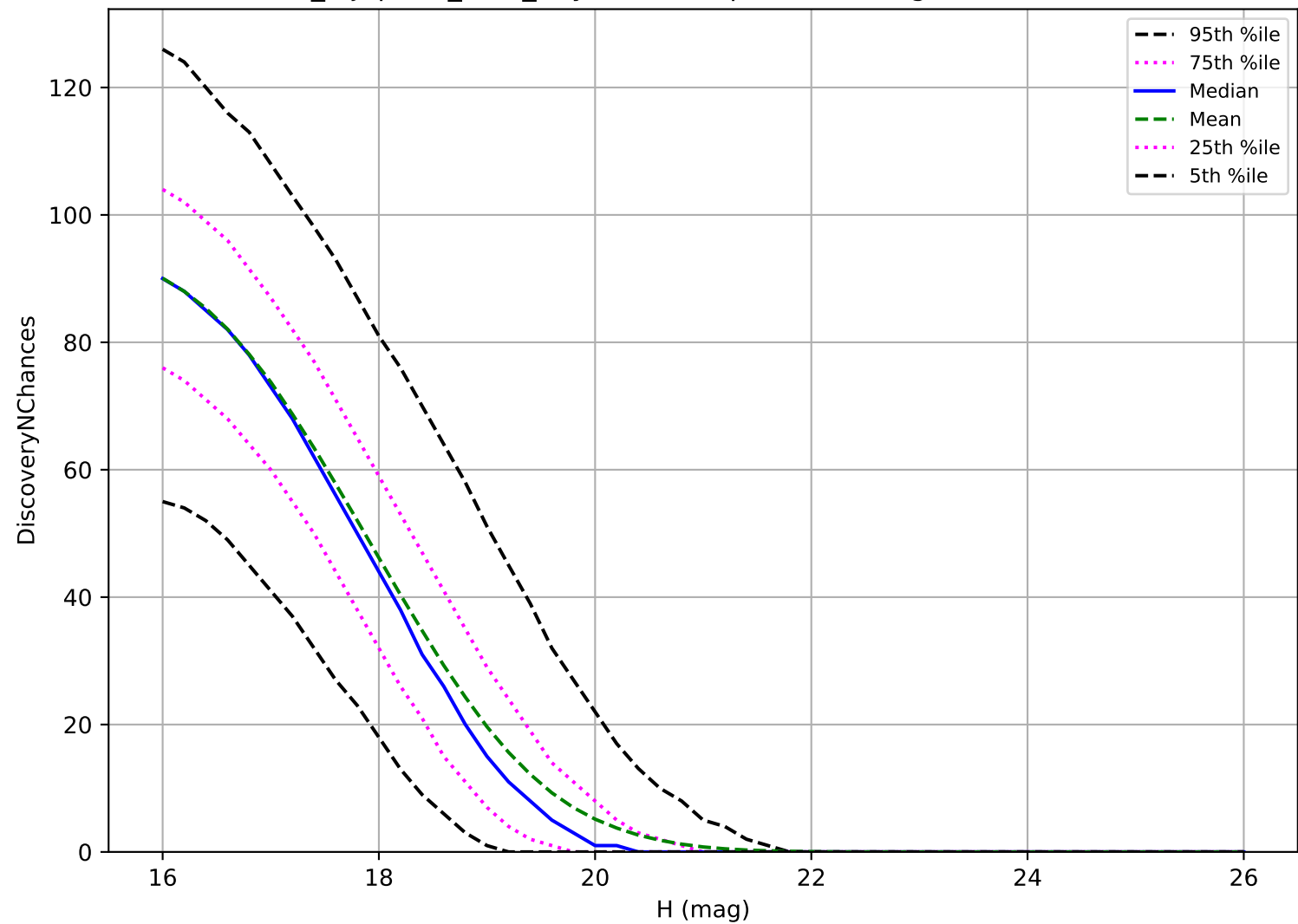
noroll_mjdp270_v3.4_10yrs: MBA 3 pairs in 15 nights detection loss
