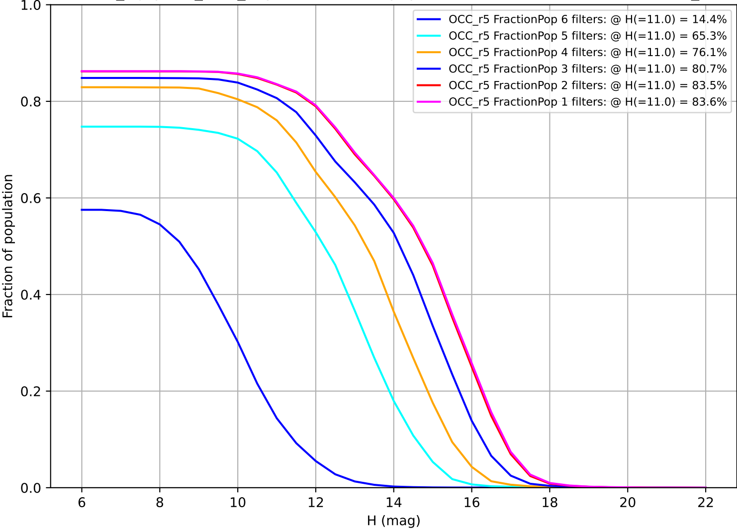
noroll_mjdp270_v3.4_10yrs: Fraction of population with colors in X filters OCC_r5
