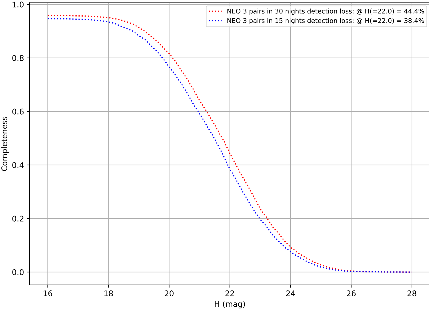
noroll_mjdp270_v3.4_10yrs: DifferentialCompleteness
