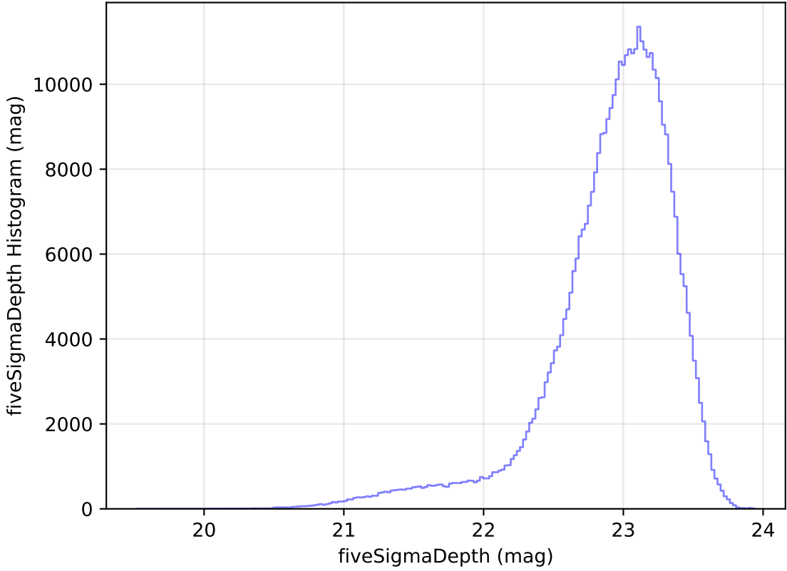
noroll_mjdp270_v3.4_10yrs z: fiveSigmaDepth Histogram
