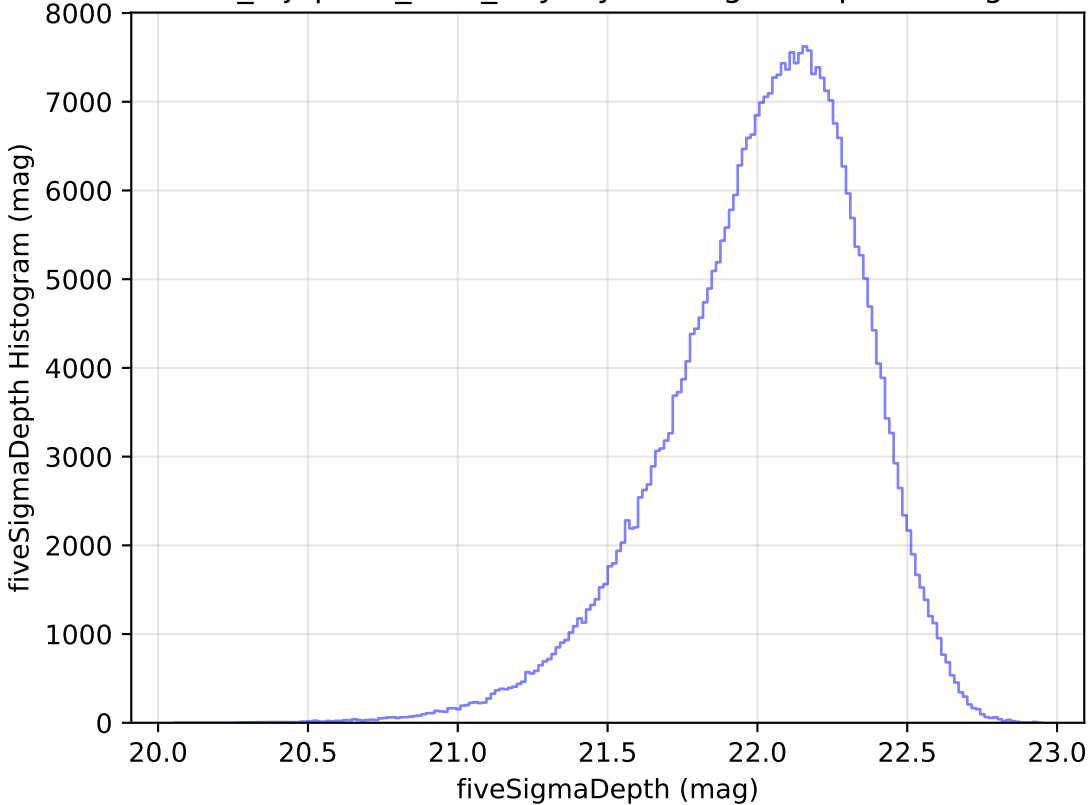
noroll_mjdp270_v3.4_10yrs y: fiveSigmaDepth Histogram
