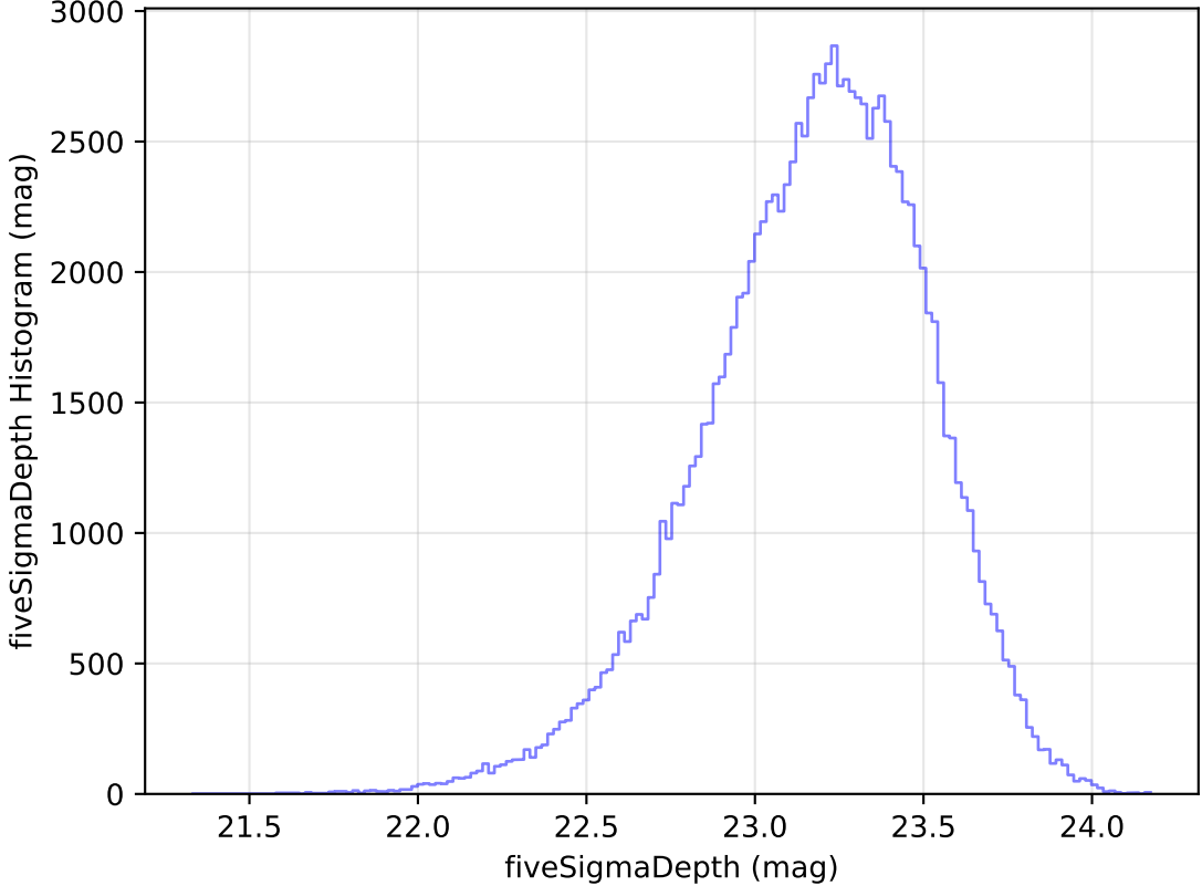
noroll_mjdp270_v3.4_10yrs u: fiveSigmaDepth Histogram
