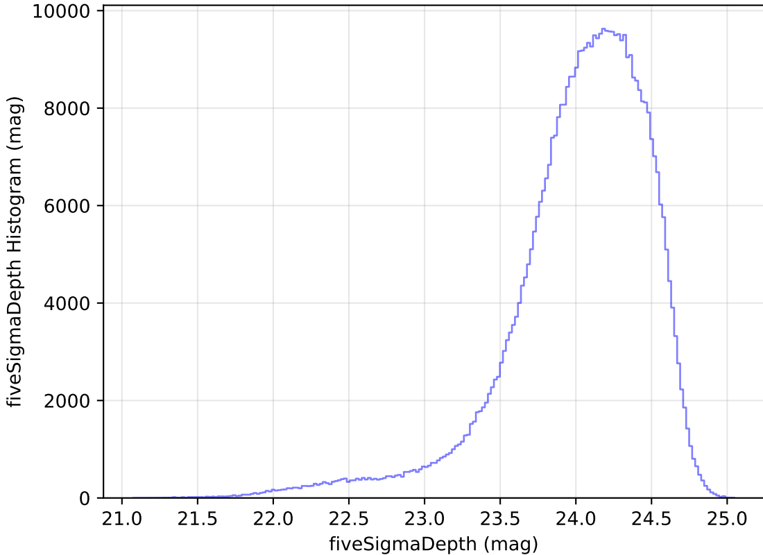
noroll_mjdp270_v3.4_10yrs r: fiveSigmaDepth Histogram
