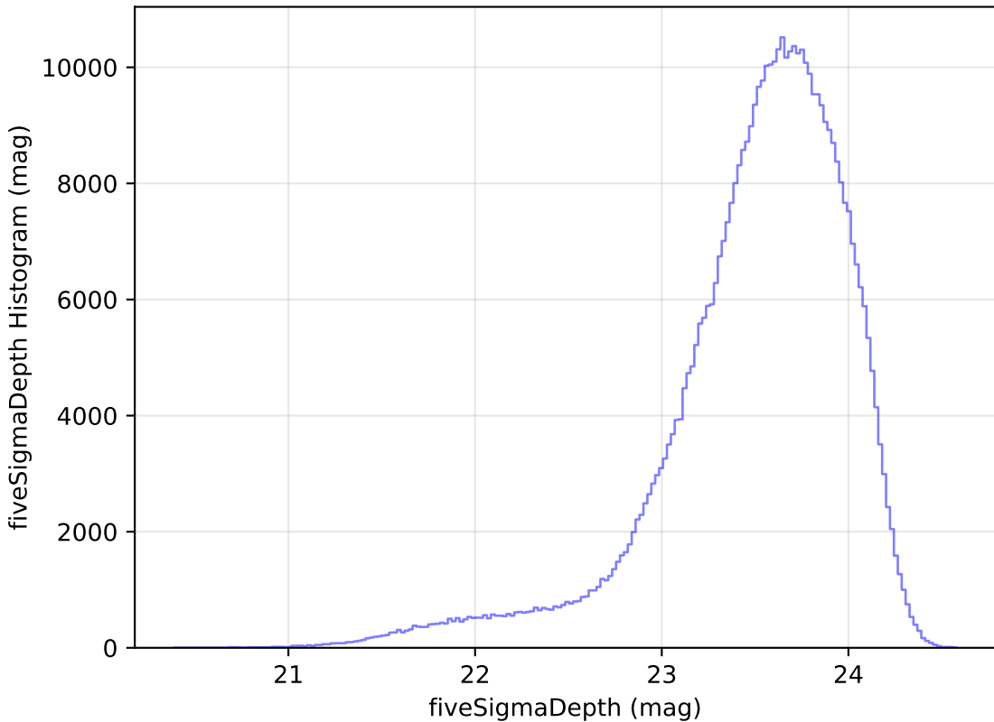
noroll_mjdp270_v3.4_10yrs i: fiveSigmaDepth Histogram
