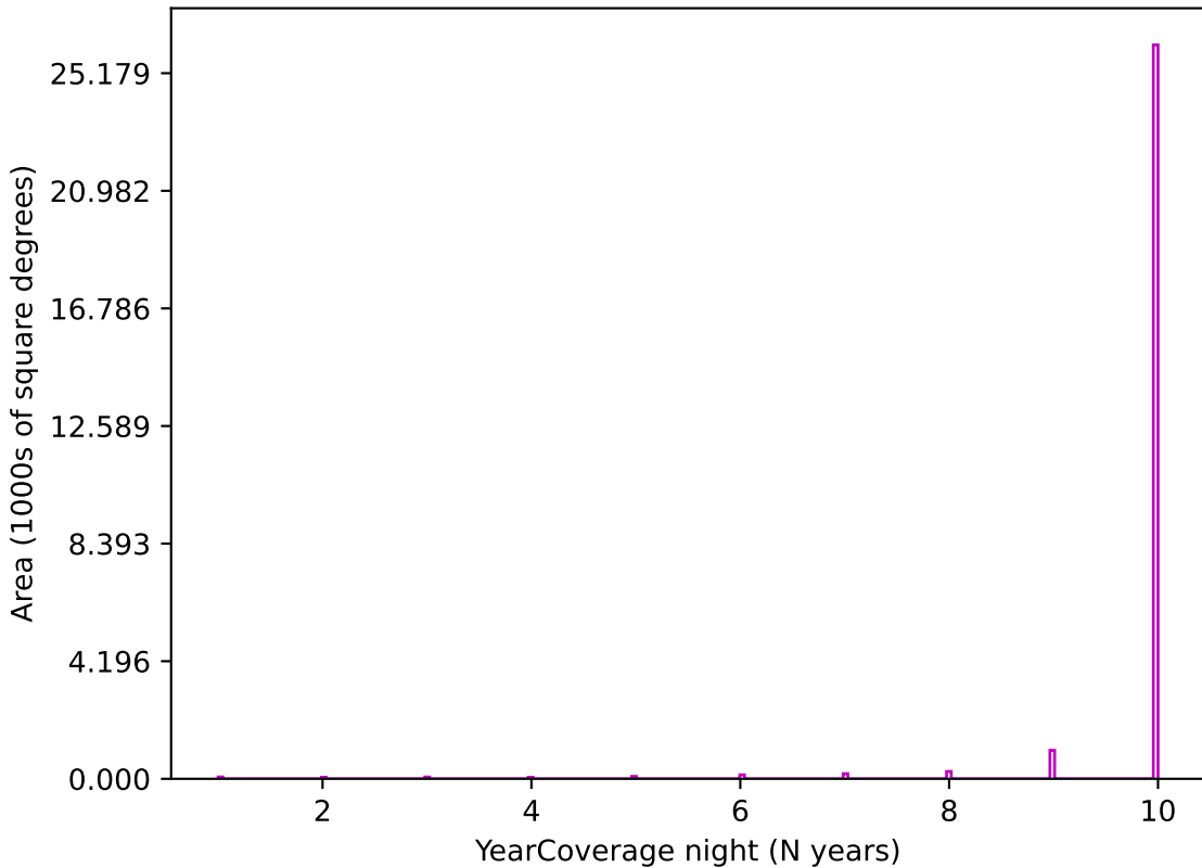
noroll_mjdp270_v3.4_10yrs z band: YearCoverage night
