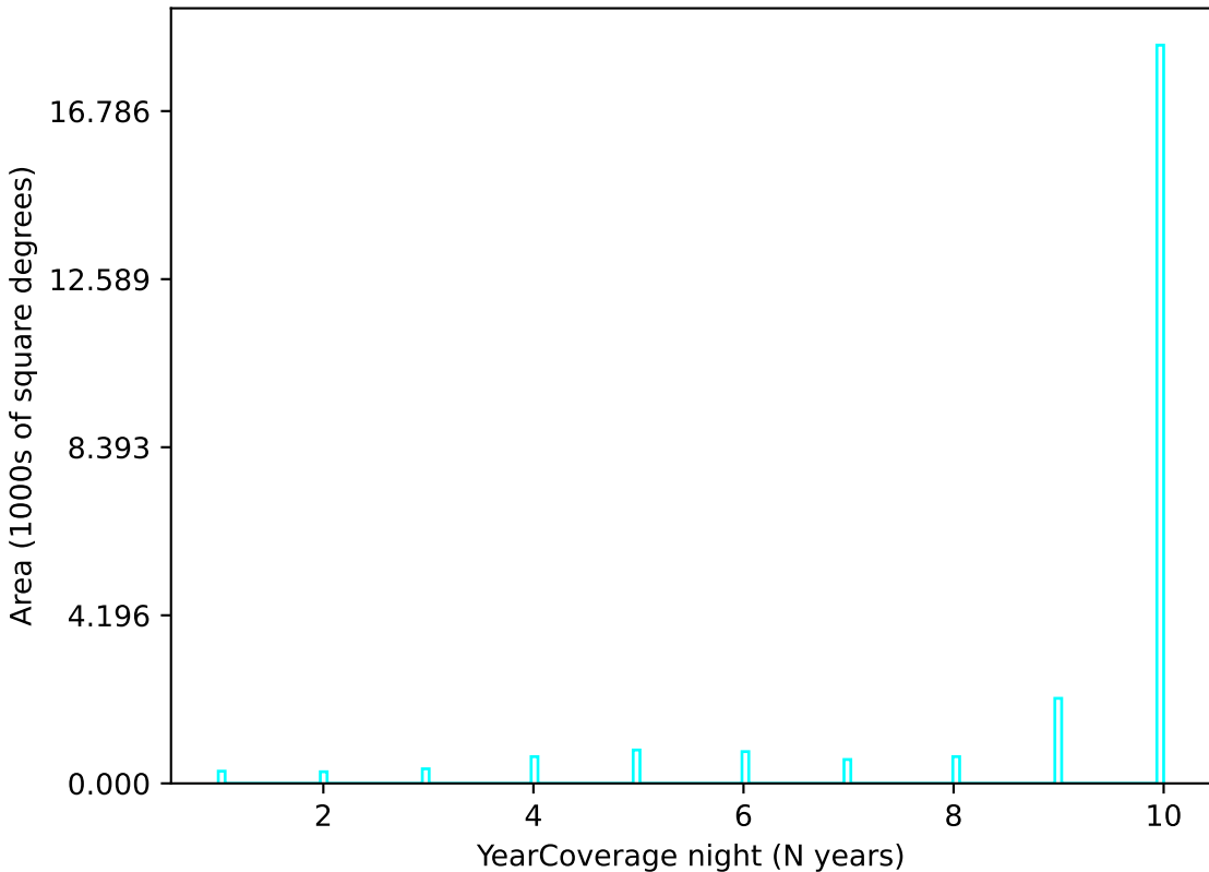
noroll_mjdp270_v3.4_10yrs u band: YearCoverage night
