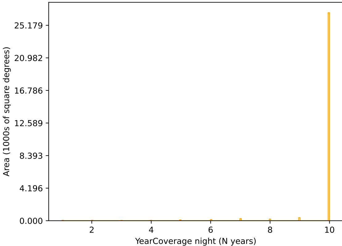
noroll_mjdp270_v3.4_10yrs r band: YearCoverage night
