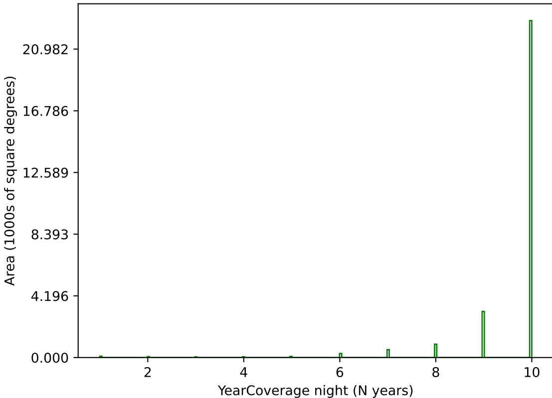
noroll_mjdp270_v3.4_10yrs g band: YearCoverage night
