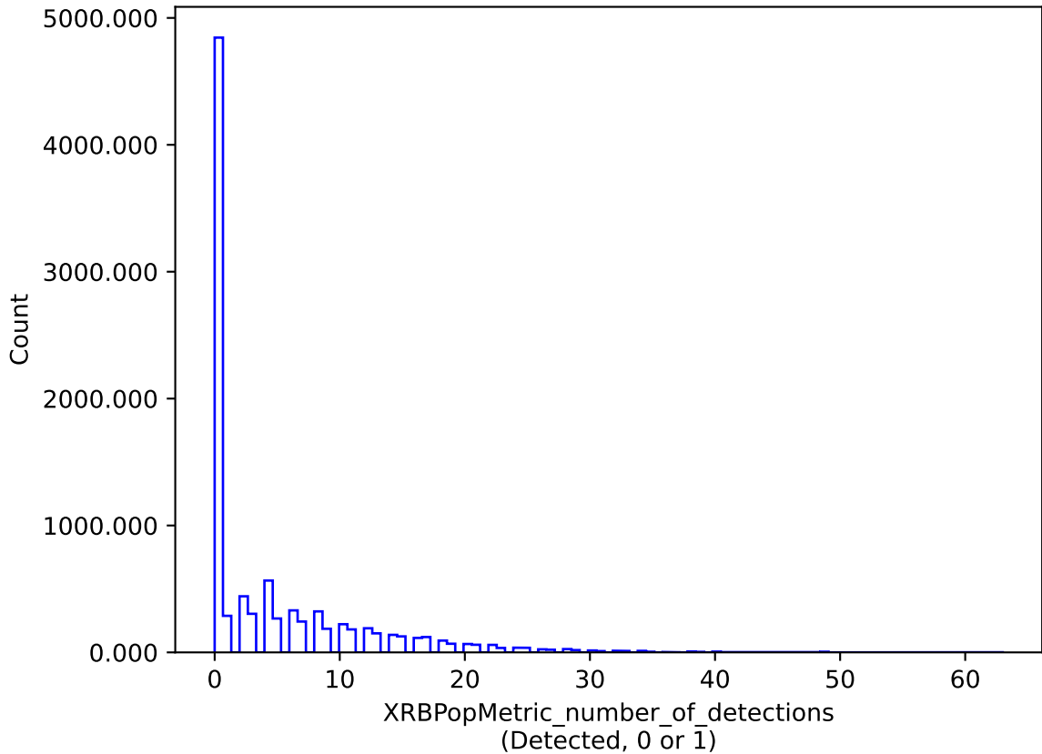
noroll_mjdp270_v3.4_10yrs : XRBPoMetric_number_of_detections
