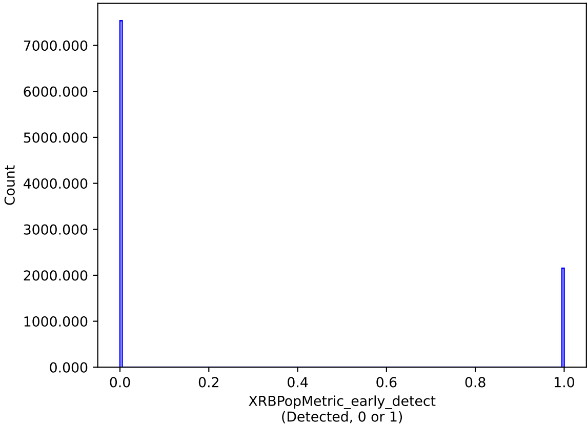
noroll_mjdp270_v3.4_10yrs : XRBPopMetric_early_detect
