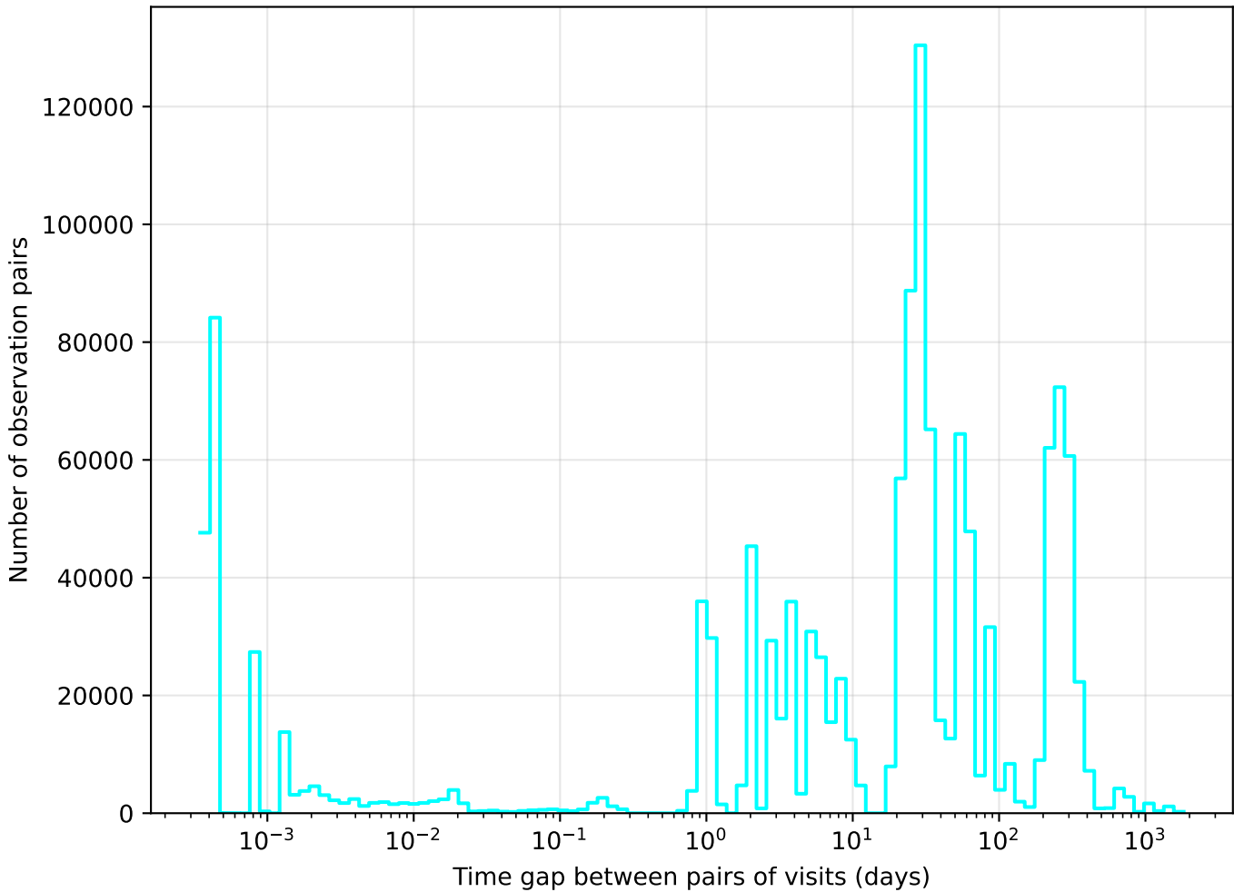
noroll_mjdp270_v3.4_10yrs u band: Tgaps observationStartMJD
