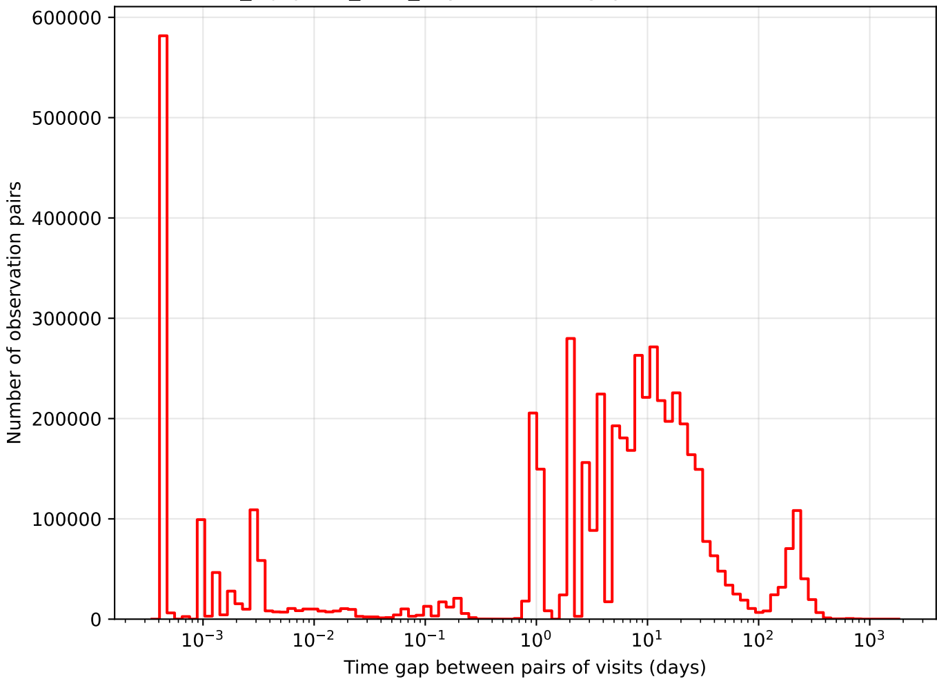
noroll_mjdp270_v3.4_10yrs i band: Tgaps observationStartMJD
