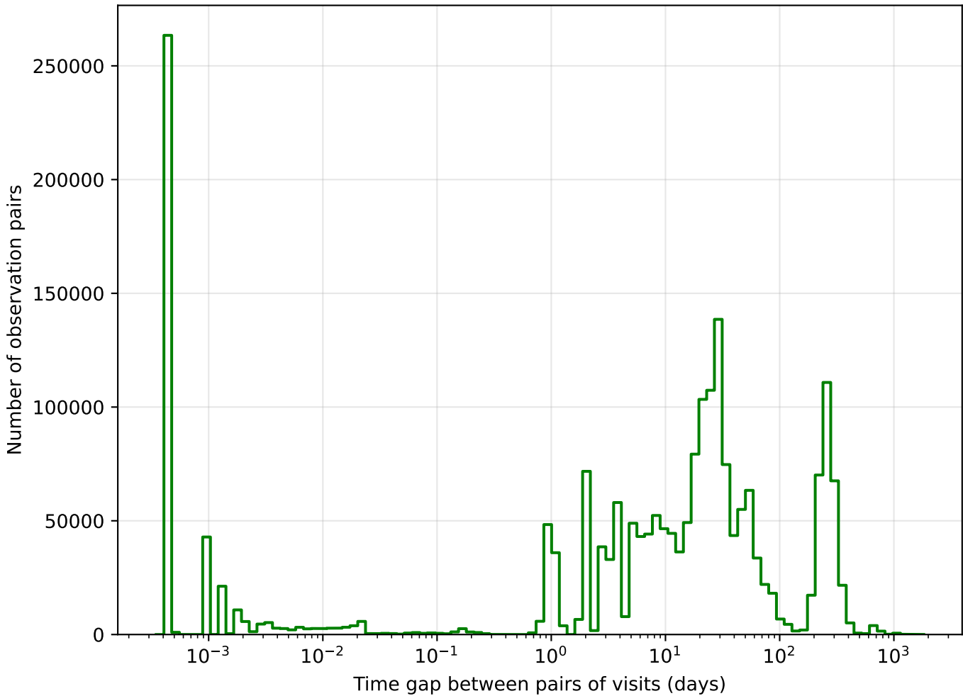
noroll_mjdp270_v3.4_10yrs g band: Tgaps observationStartMJD
