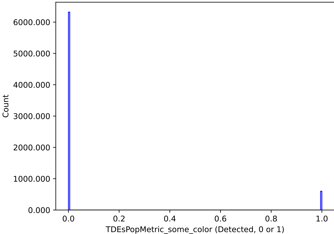
noroll_mjdp270_v3.4_10yrs : TDEsPopMetric_some_color
