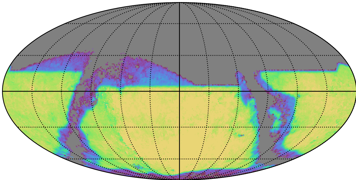
noroll_mjdp270_v3.4_10yrs : TDC_rate
