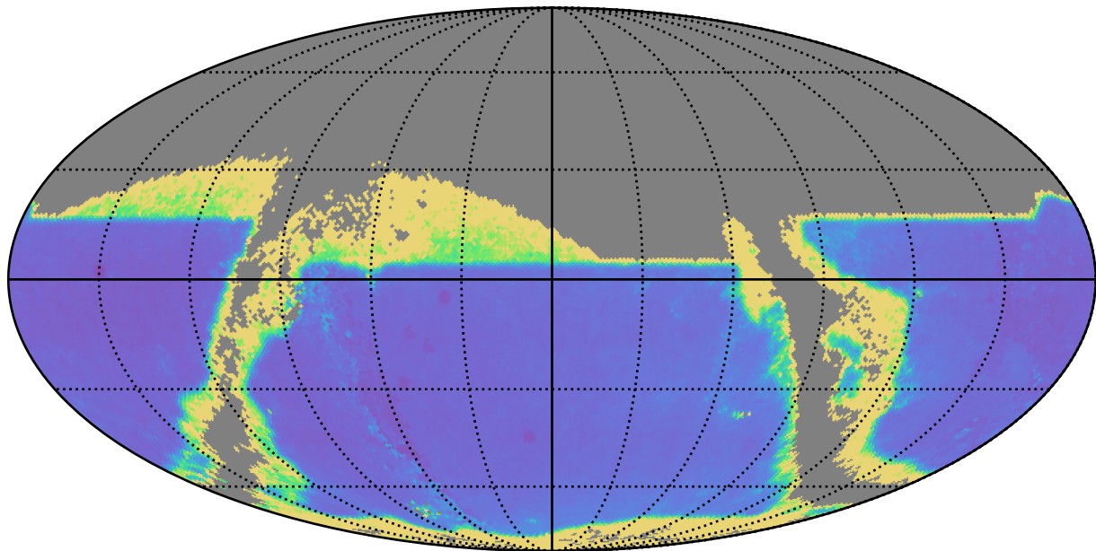
noroll_mjdp270_v3.4_10yrs : TDC_precision
