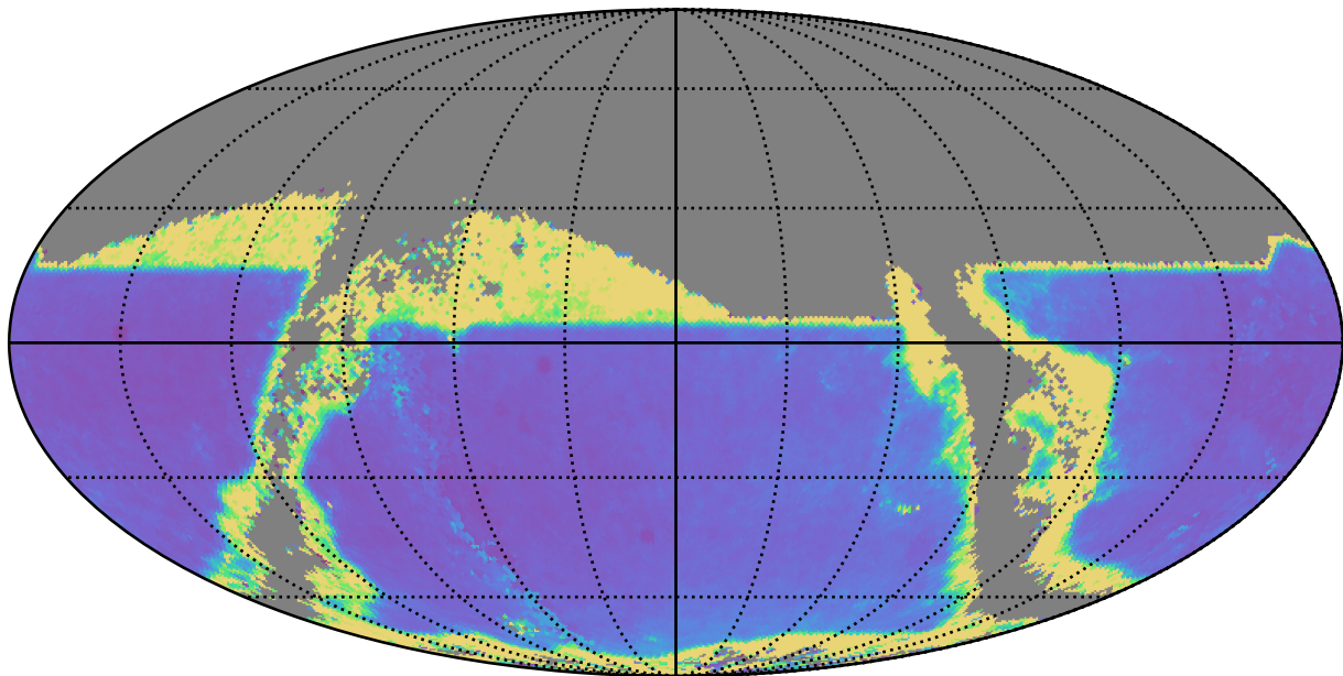
noroll_mjdp270_v3.4_10yrs : TDC_cadence
