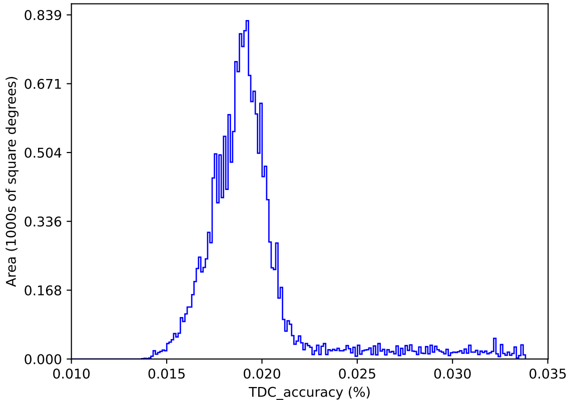
noroll_mjdp270_v3.4_10yrs : TDC_accuracy
