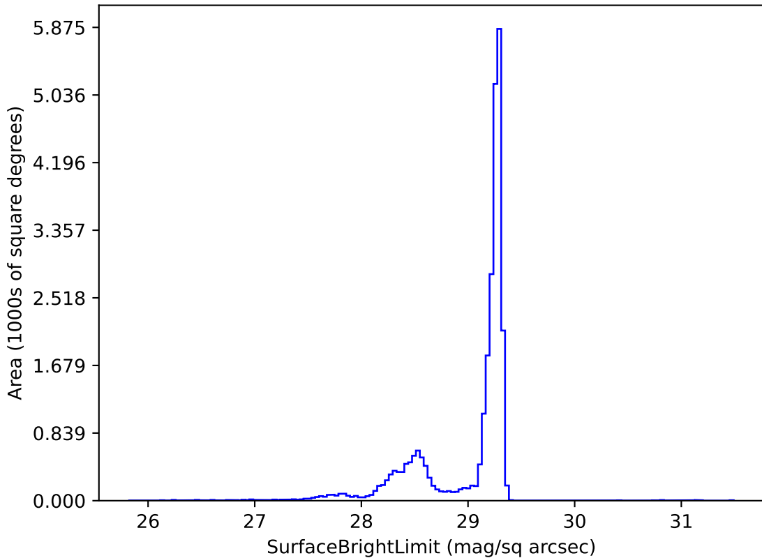
noroll_mjdp270_v3.4_10yrs z: SurfaceBrightLimit
