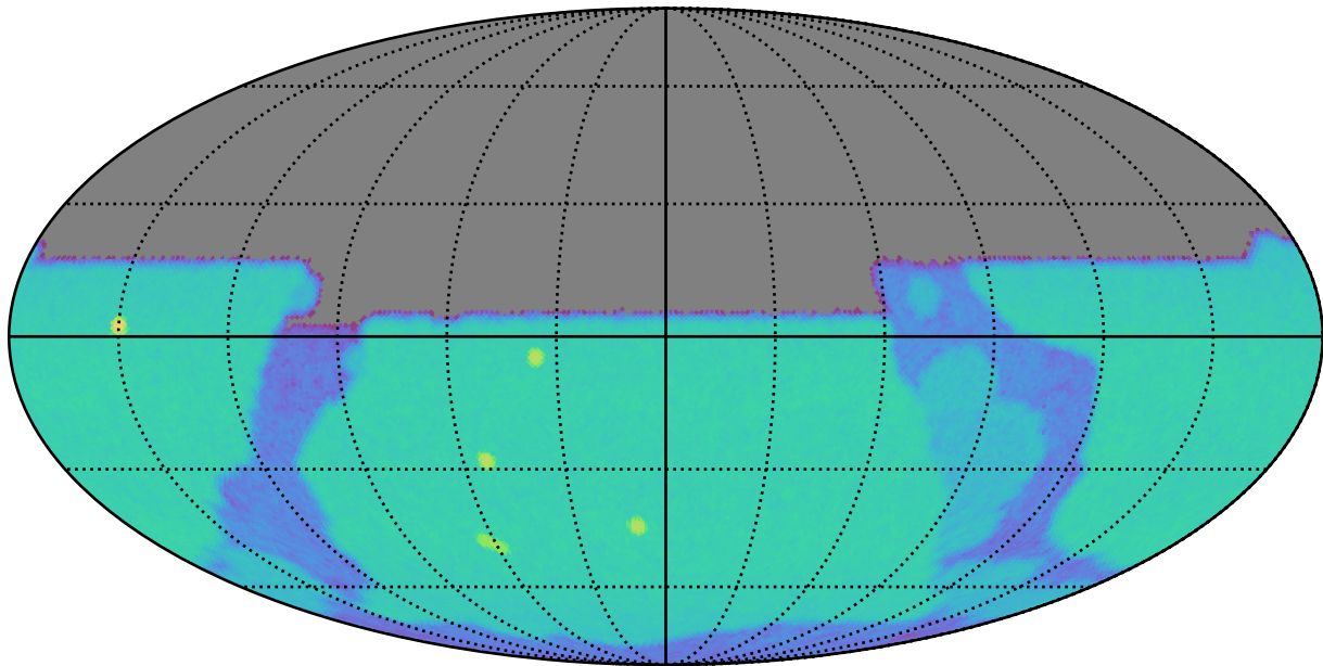
noroll_mjdp270_v3.4_10yrs u: SurfaceBrightLimit
