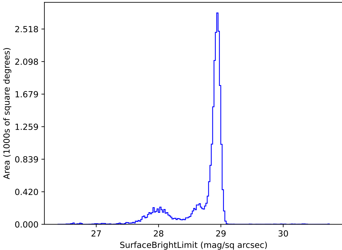
noroll_mjdp270_v3.4_10yrs u: SurfaceBrightLimit
