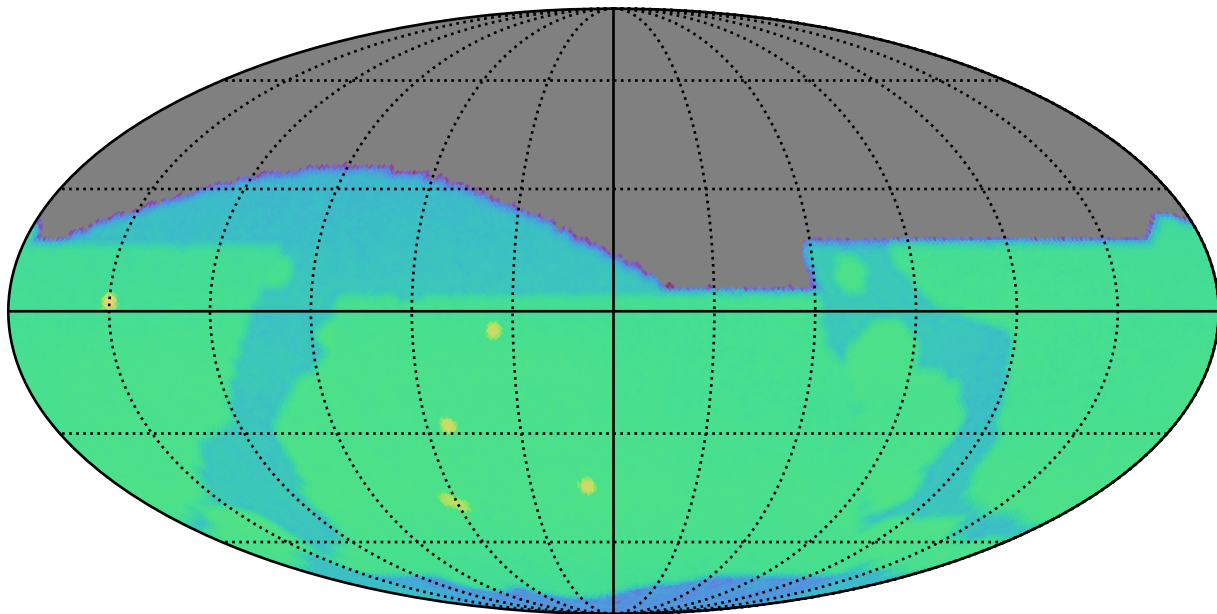
noroll_mjdp270_v3.4_10yrs r: SurfaceBrightLimit
