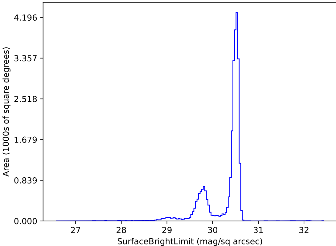
noroll_mjdp270_v3.4_10yrs r: SurfaceBrightLimit
