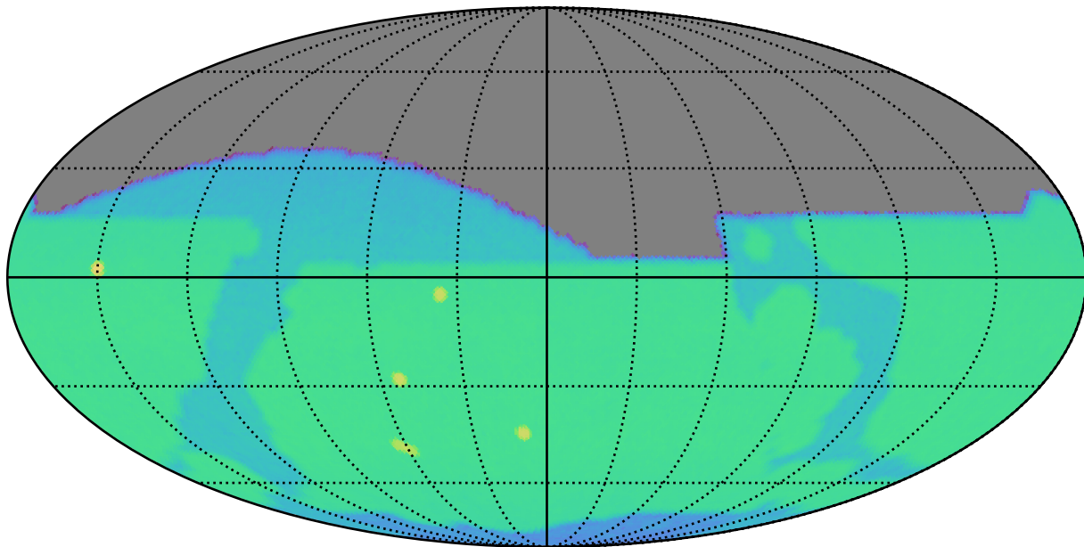
noroll_mjdp270_v3.4_10yrs i: SurfaceBrightLimit
