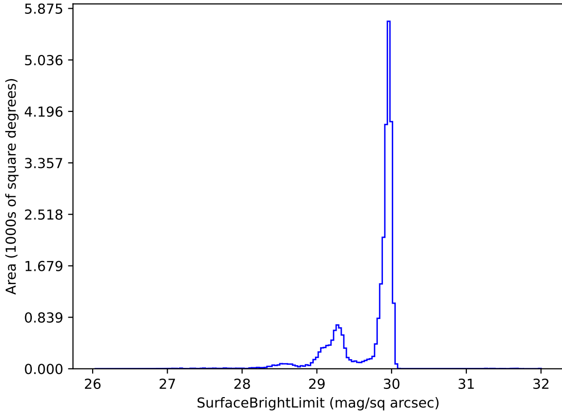
noroll_mjdp270_v3.4_10yrs i: SurfaceBrightLimit
