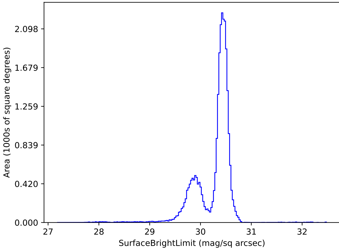
noroll_mjdp270_v3.4_10yrs g: SurfaceBrightLimit
