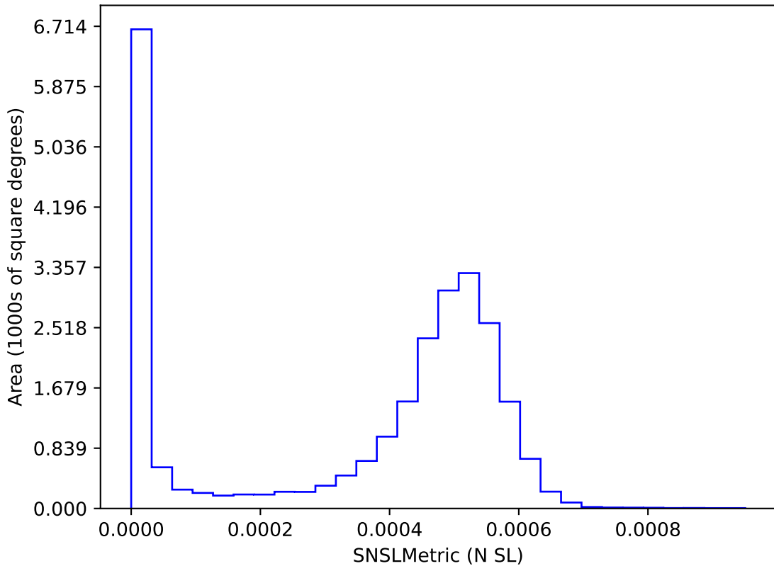
noroll_mjdp270_v3.4_10yrs : SNSLMetric
