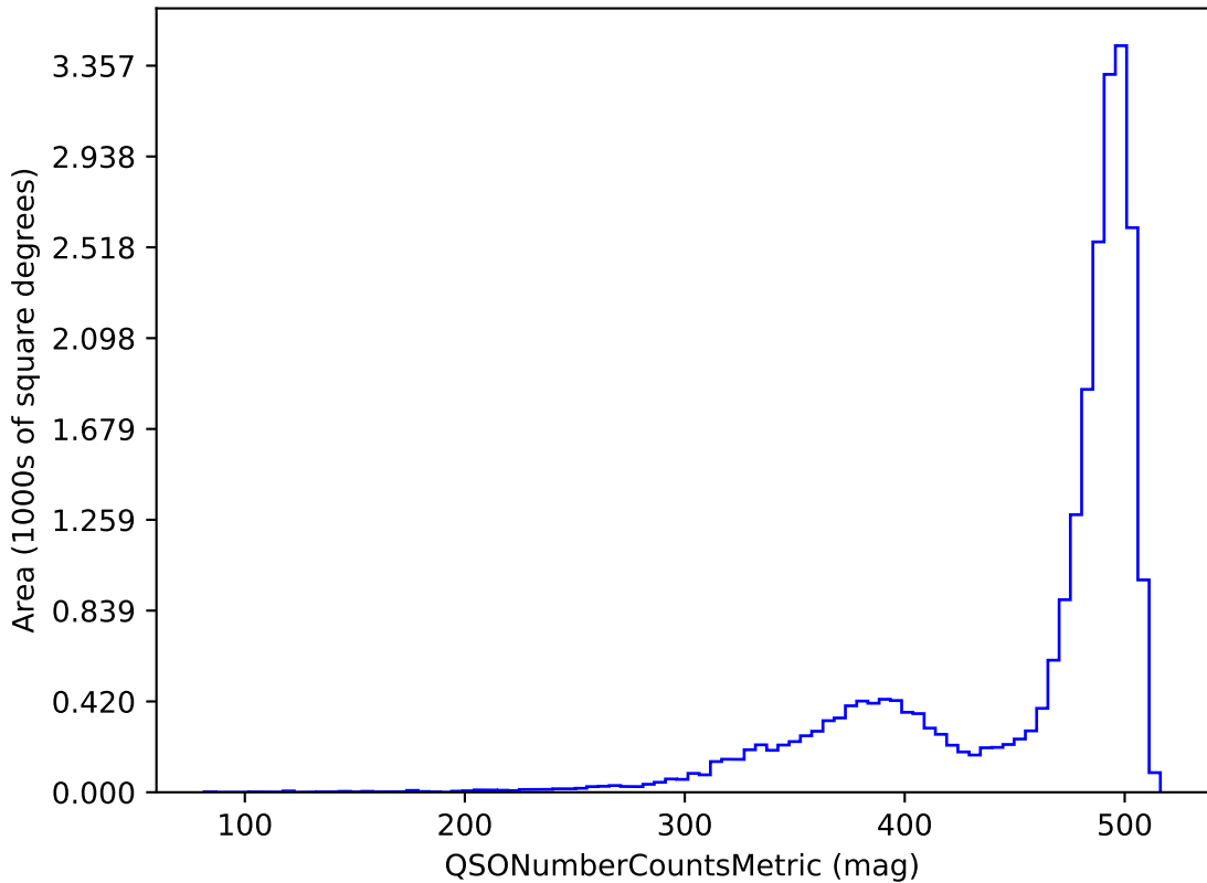
noroll_mjdp270_v3.4_10yrs z band and non-DD: QSONumberCountsMetric
