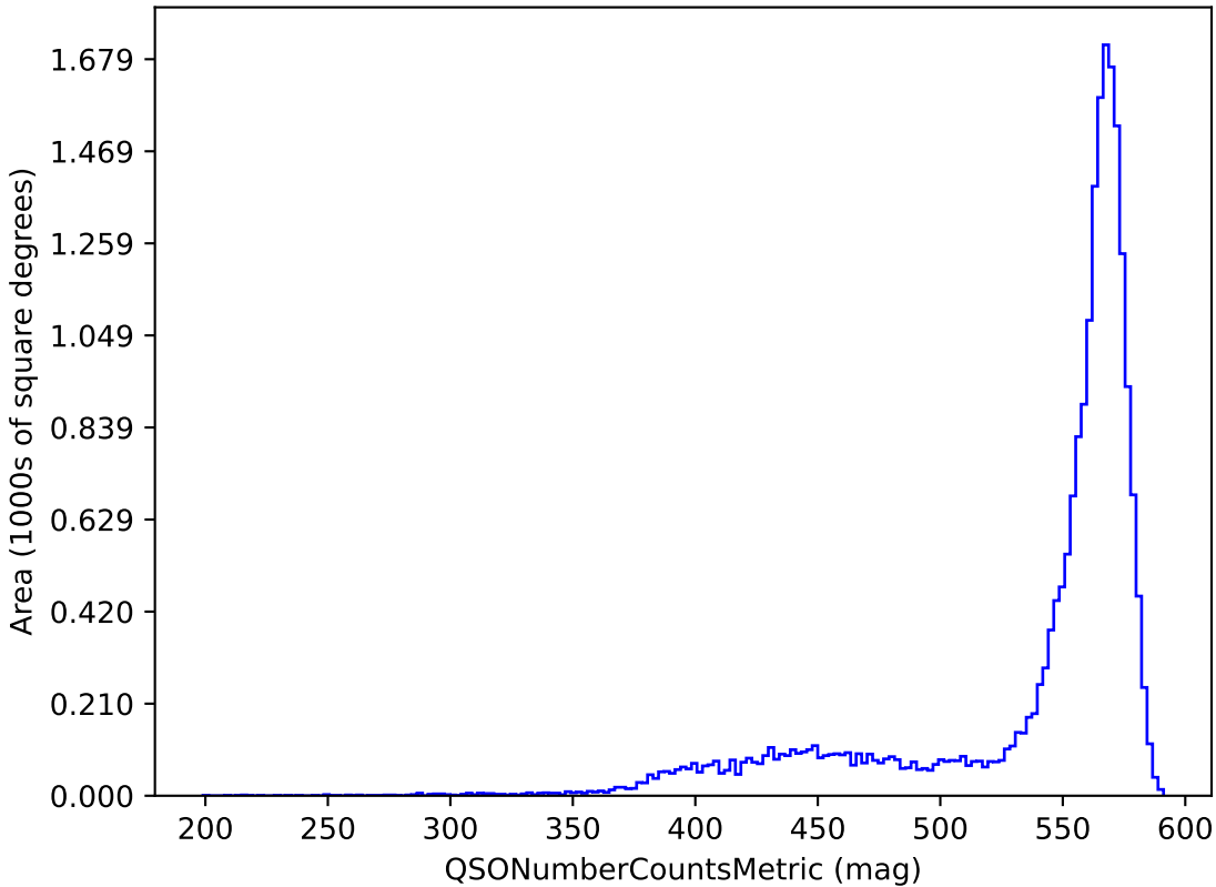
noroll_mjdp270_v3.4_10yrs y band and non-DD: QSONumberCountsMetric
