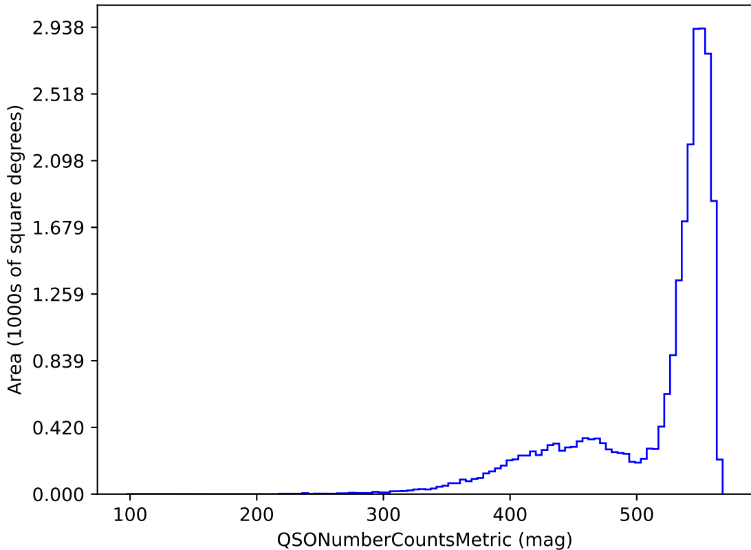
noroll_mjdp270_v3.4_10yrs i band and non-DD: QSONumberCountsMetric
