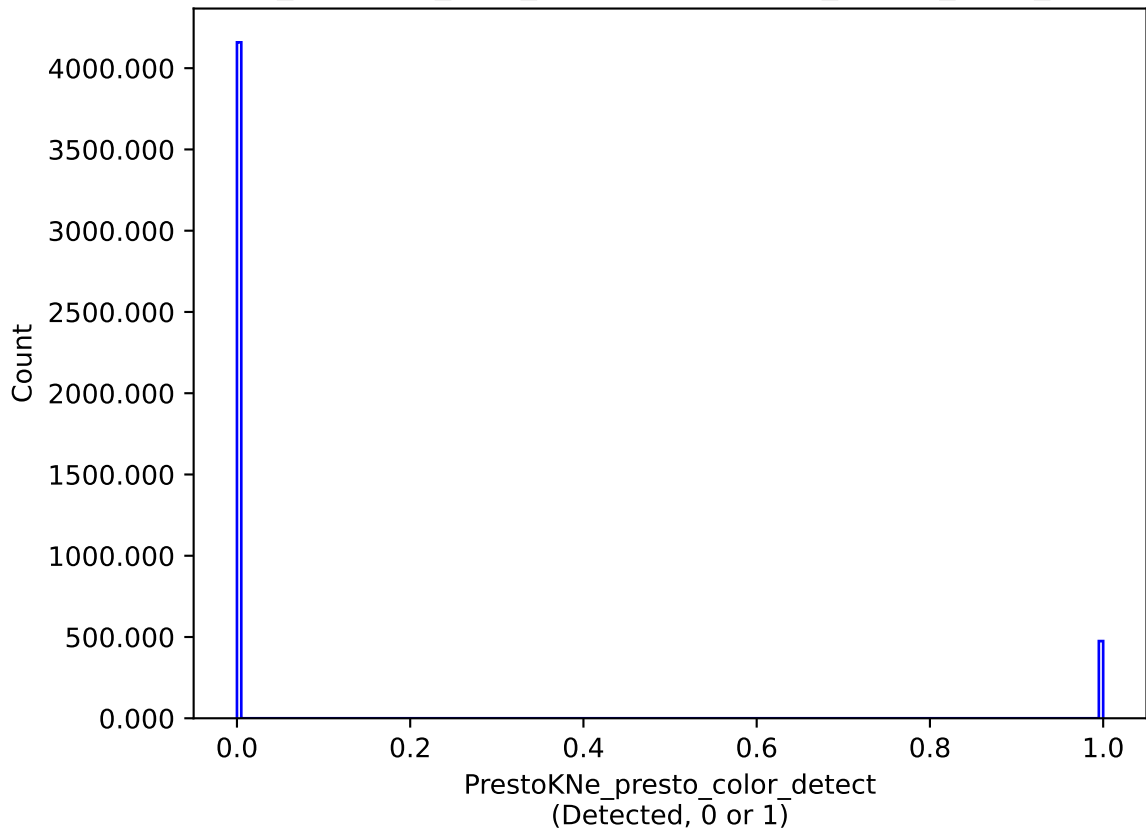
noroll_mjdp270_v3.4_10yrs : PrestoKNe_presto_color_detect
