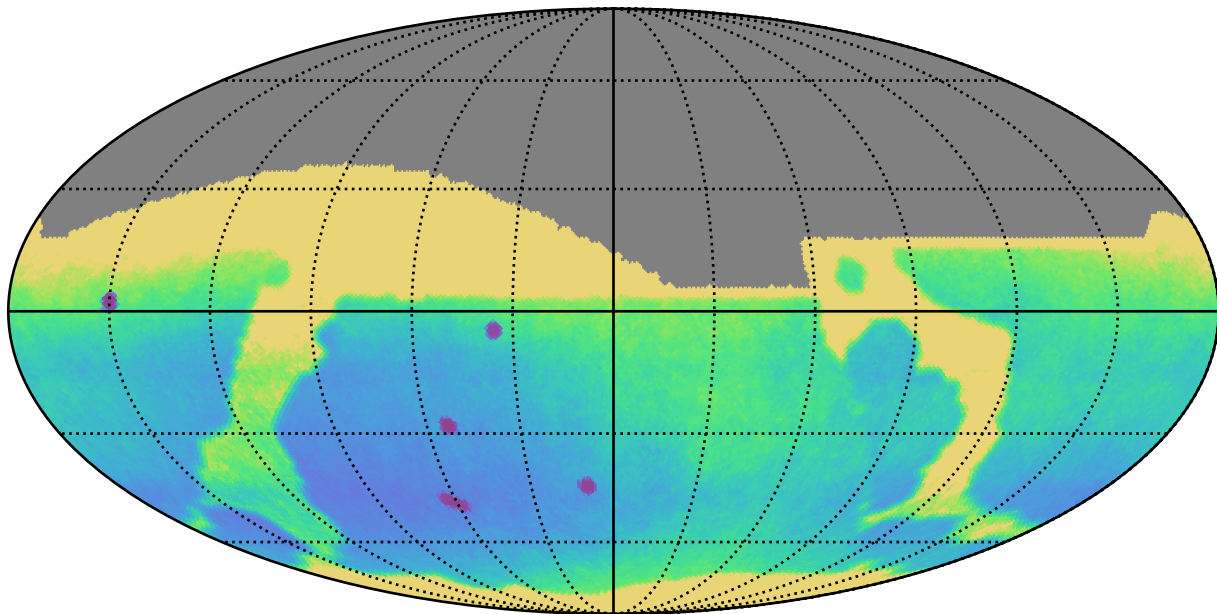
noroll_mjdp270_v3.4_10yrs : Parallax Uncert @ 24.0
