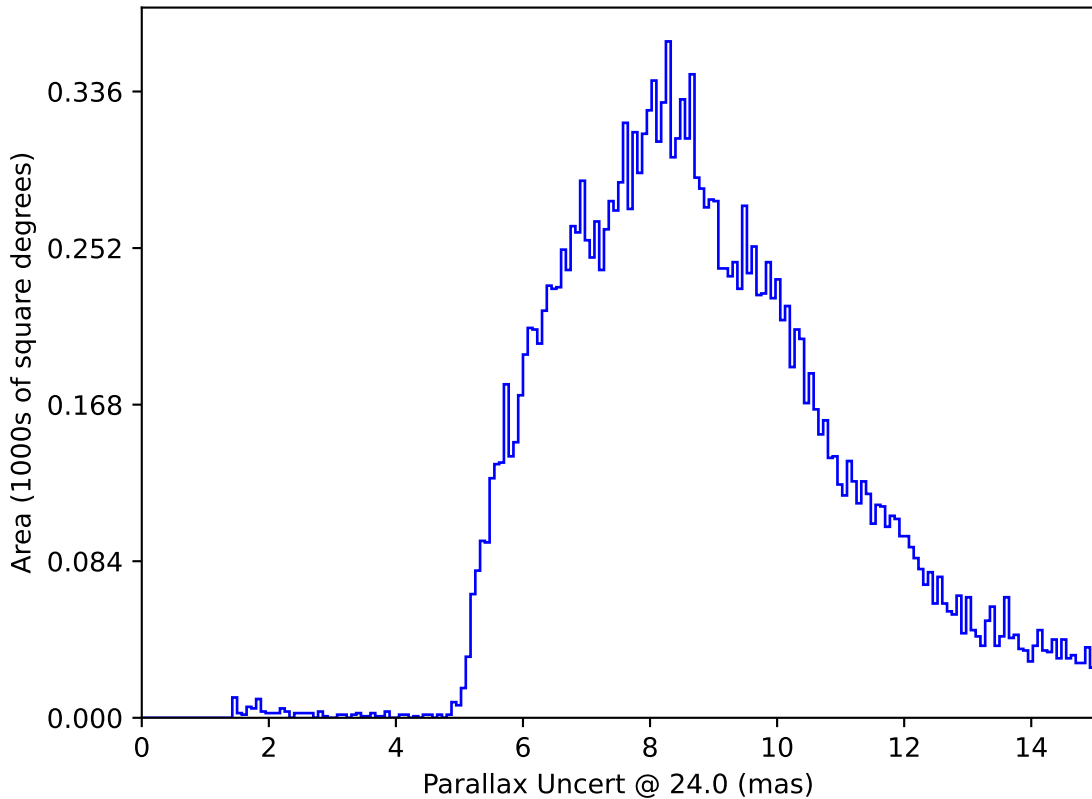
noroll_mjdp270_v3.4_10yrs : Parallax Uncert @ 24.0
